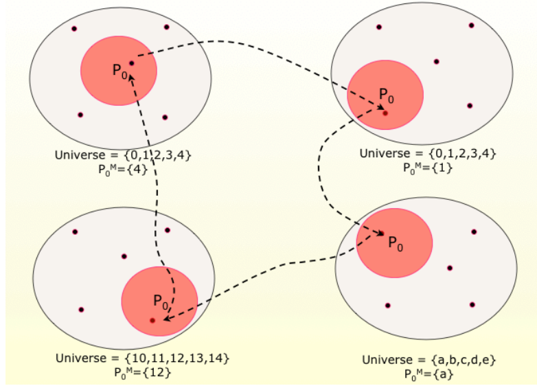
Figure 2.18: Four isomorphic unary structures.
