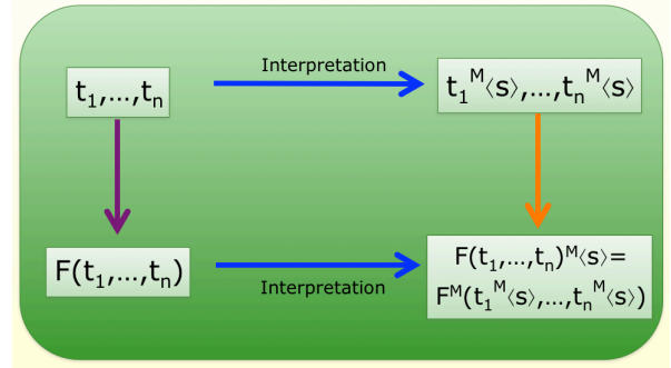
Figure 2.15: The value of a term.
