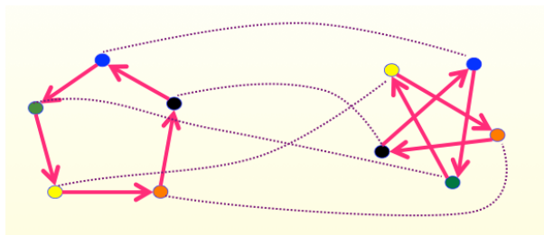
Figure 2.20: Isomorphism of unary functions.
