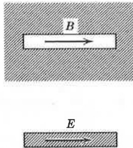
Fig. 9.13 Equivalent radiators according to Babinet's principle.
