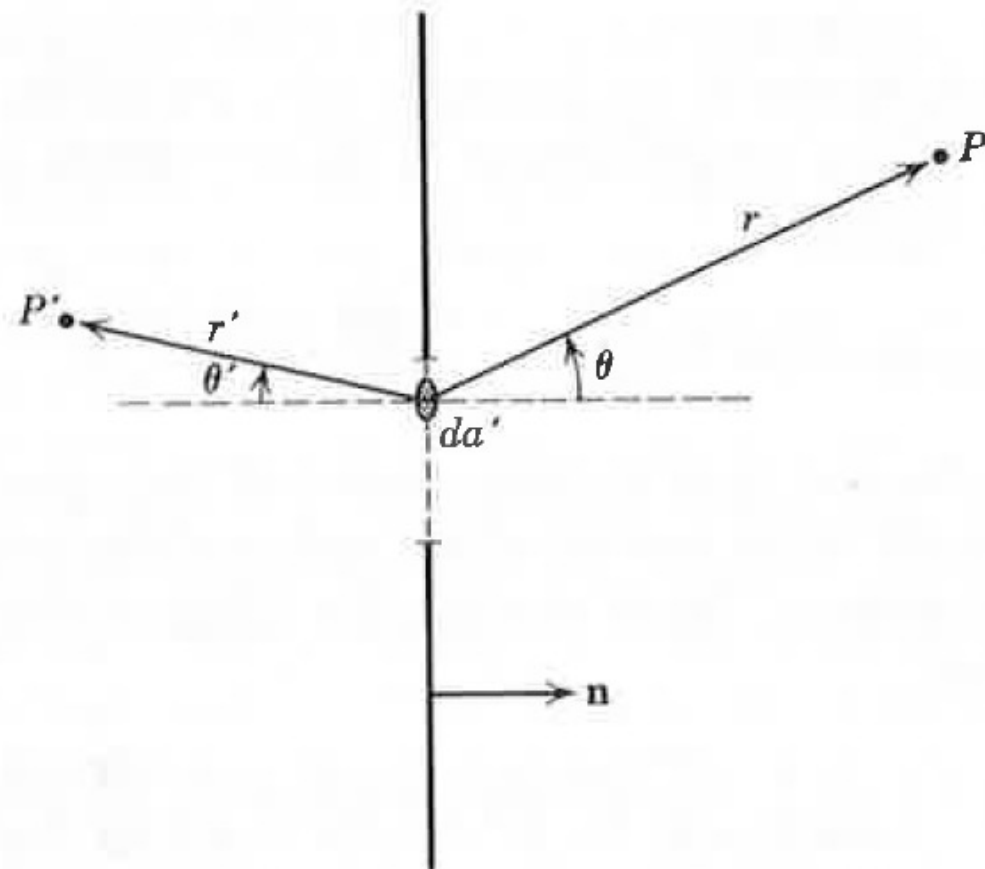
Fig. 9.10 Diffraction geometry for a point source at P' , a plane screen with apertures, and an observation point at P . The distances from the element of area da' in the aperture to the points P and P' are r and r' , respectively. The angles \theta and \theta' are those between \mathbf{r} and \mathbf{n} , and \mathbf{r}' and -\mathbf{n} , respectively.
