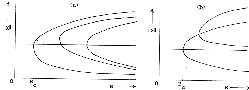
Figure 3. Repeated branching.
