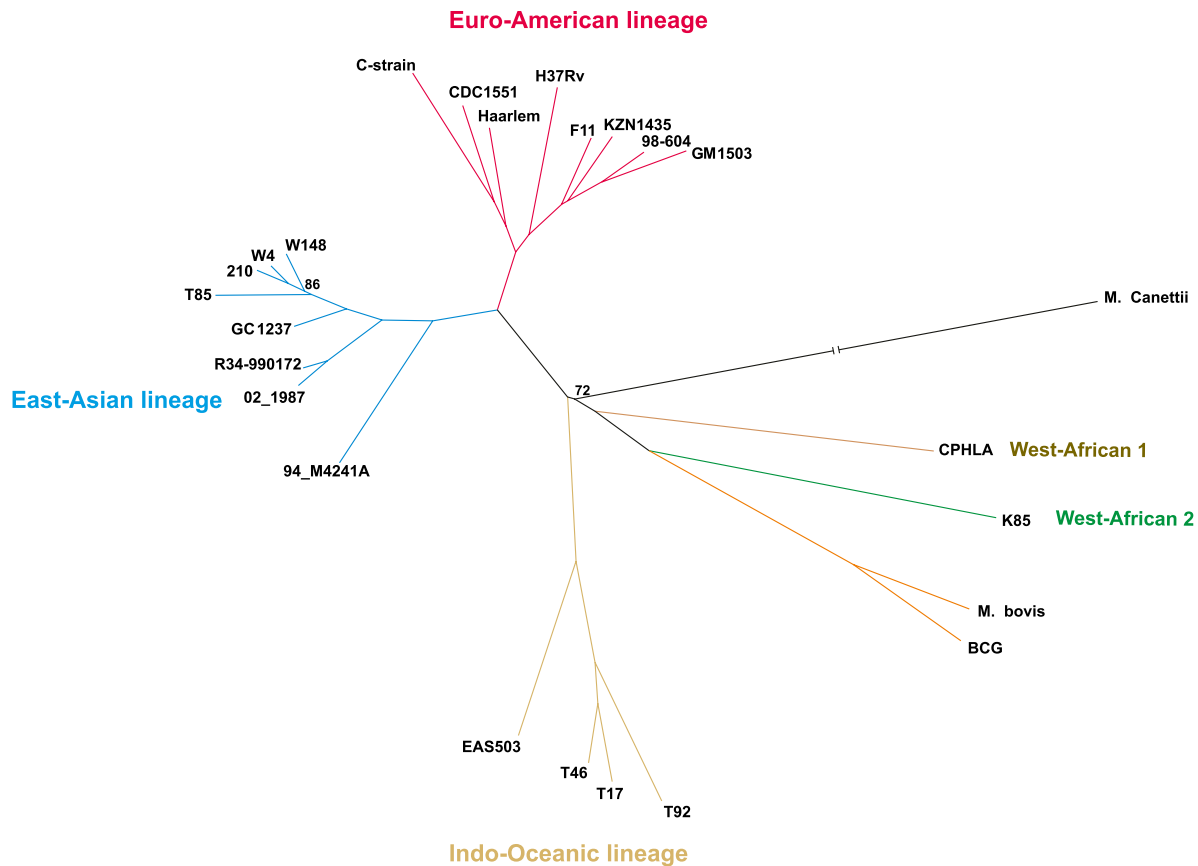
Figure 1. Phylogenetic tree constructed using SNPs purged of recombination tracts. The maximum likelihood tree was constructed using RaxML v7.2.8. Only nodes with bootstrap support values below 100% are indicated.
