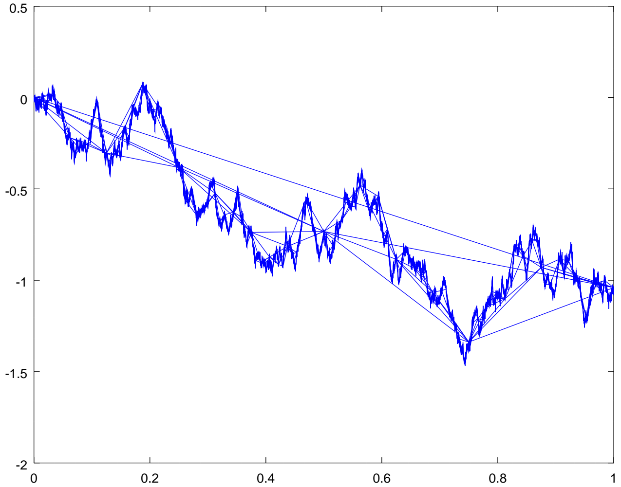
Levy construction of Brownian path on the dyadics at level14
