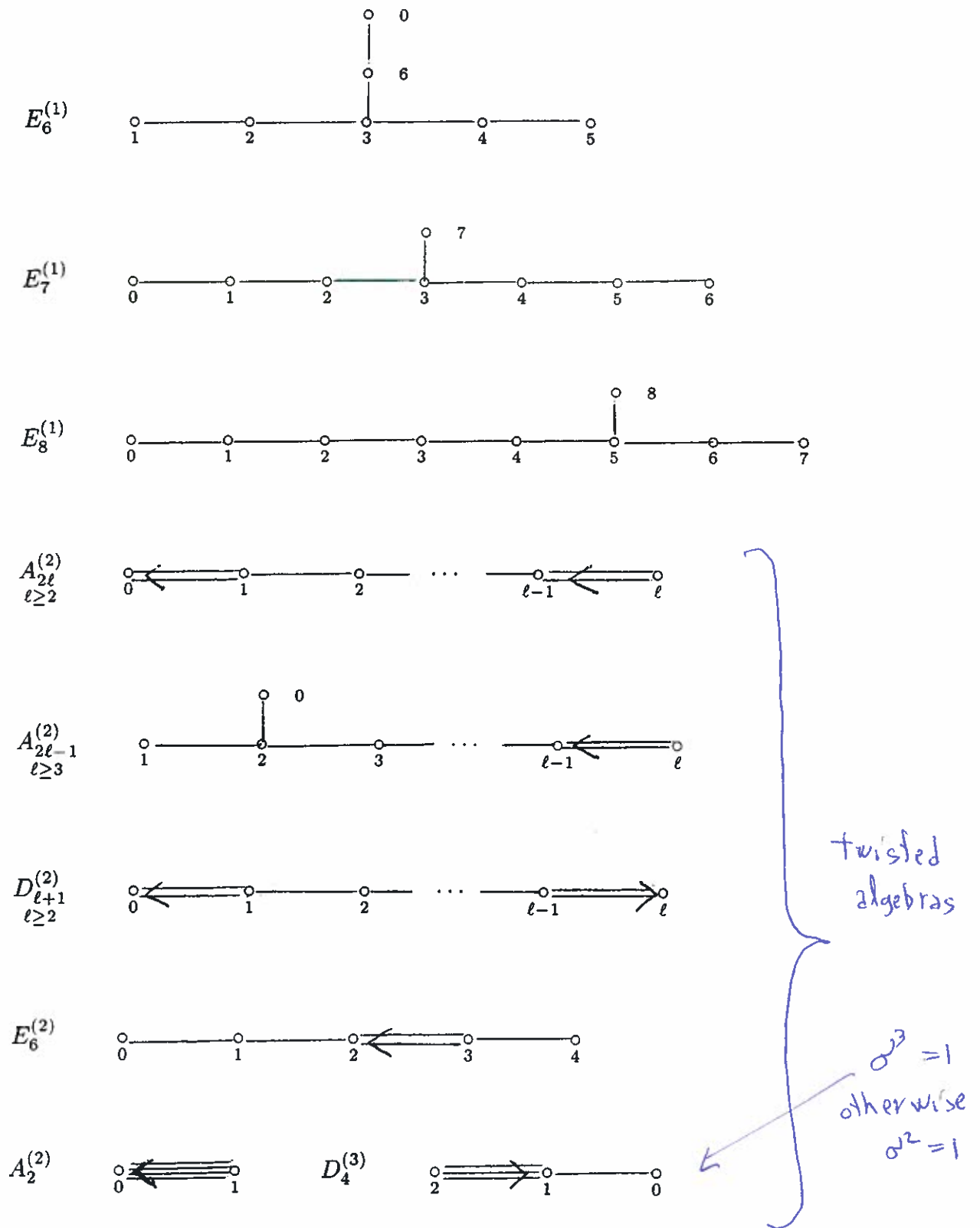
Figure Aff2 Dynkin diagrams for affine Lie algebras.
