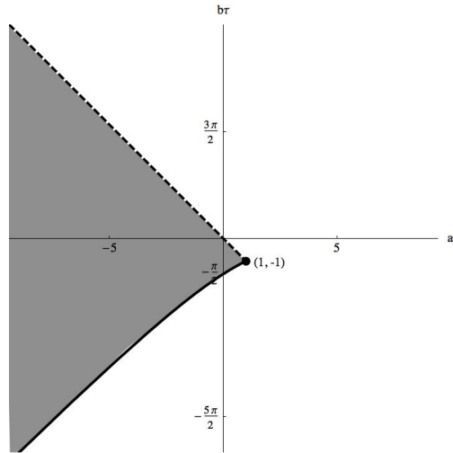
FIGURE 2. Stability (grey) and instability (white).
