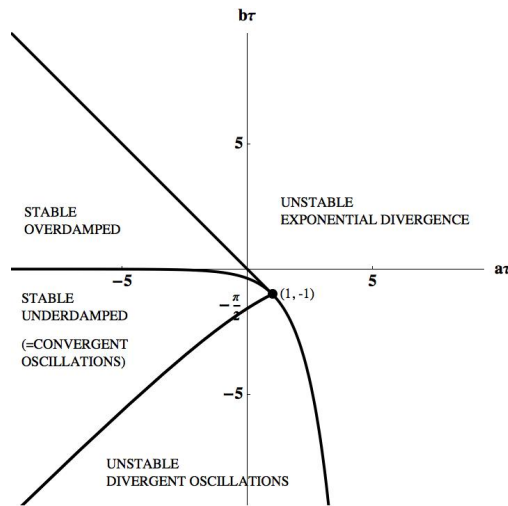
FIGURE 4. Stability boundaries for the system \frac{du}{dt} = au + bu_\tau .
