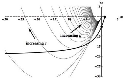
FIGURE 7. The effect of the delay \tau and the density-independent egg mortality \beta on (a\tau, b\tau) . Changes in \tau cause a movement along the (thin) curves, while changes in \beta cause a movement across the curves as indicated.
