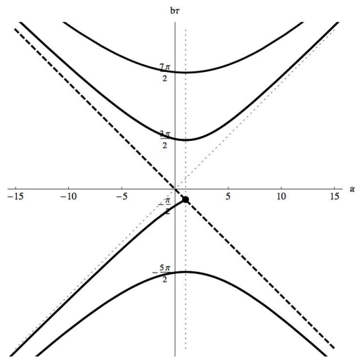
FIGURE 1. Values of (a\tau, b\tau) for which there exists a pair of complex eigenvalues exactly on the imaginary axis (solid bold lines) or for which there exists a real eigenvalue equal to zero (dashed bold line). The point (1, -1) is indicated with a solid circle.
