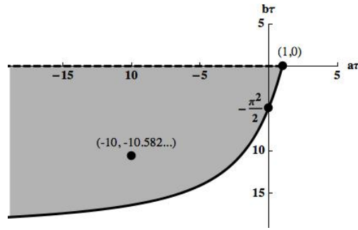
FIGURE 6. Stability (grey) and instability (white). Only the negative quadrant can be interpreted in the cannibalism model.
