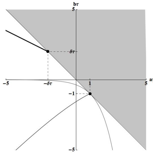
FIGURE 5. Stability in the delayed logistic \frac{dx}{dt} = \beta x_\tau e^{-\int_0^\tau \alpha(s) ds} - \delta x - \frac{1}{2}\gamma x^2 . For points (a\tau, b\tau) inside the grey region no positive equilibrium exists.
