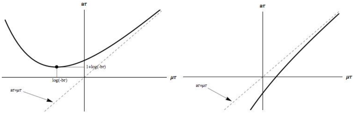
FIGURE 3. Graph of a\tau as a function of \mu\tau for fixed b\tau > 0 (left) and b\tau \leq 0 (right).
