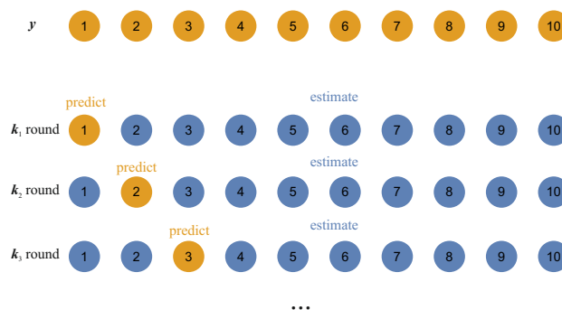
Figure 8.6: Leave-one-out crossvalidation.
