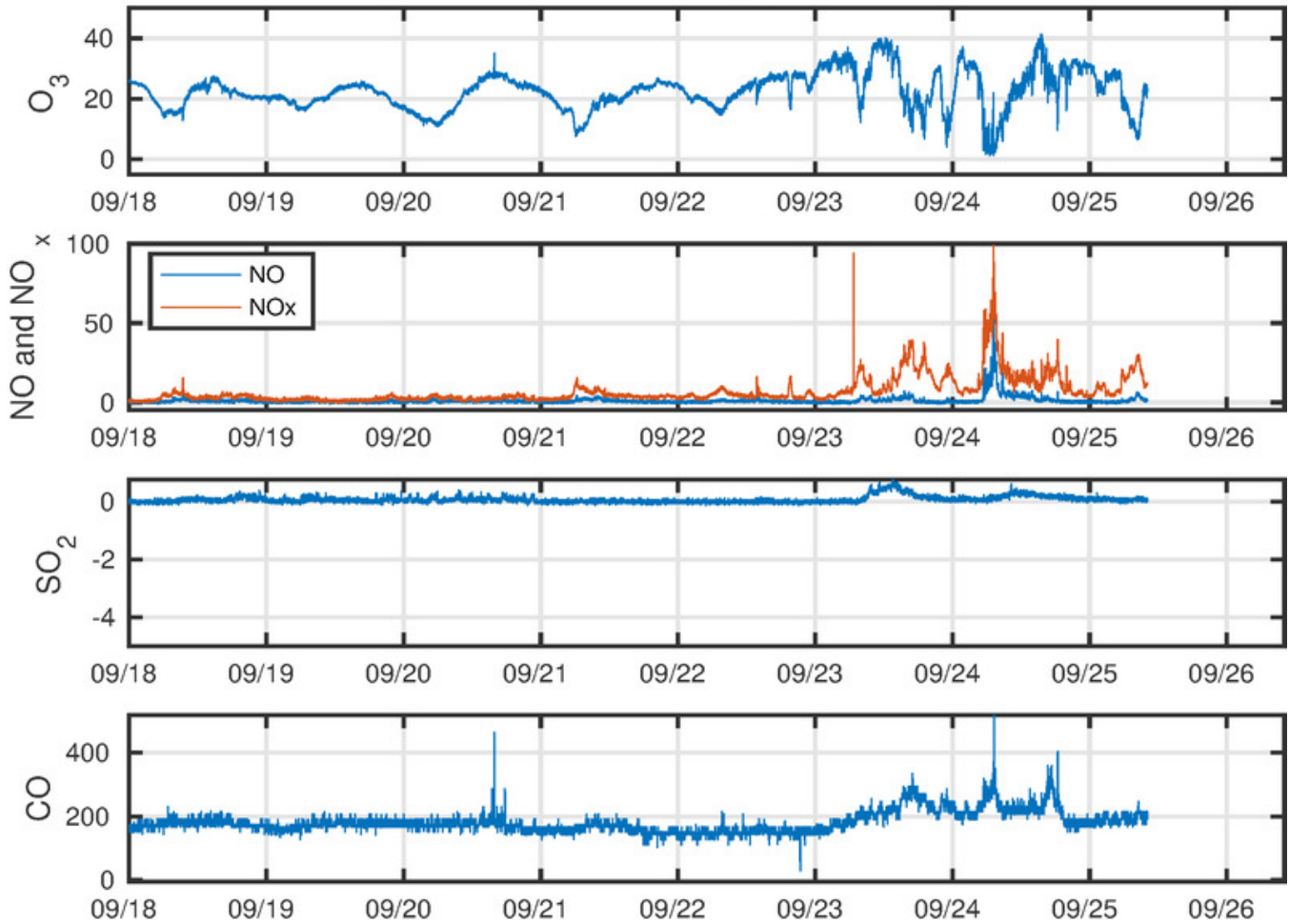
Trace gas concentrations (ppb) in Helsinki
