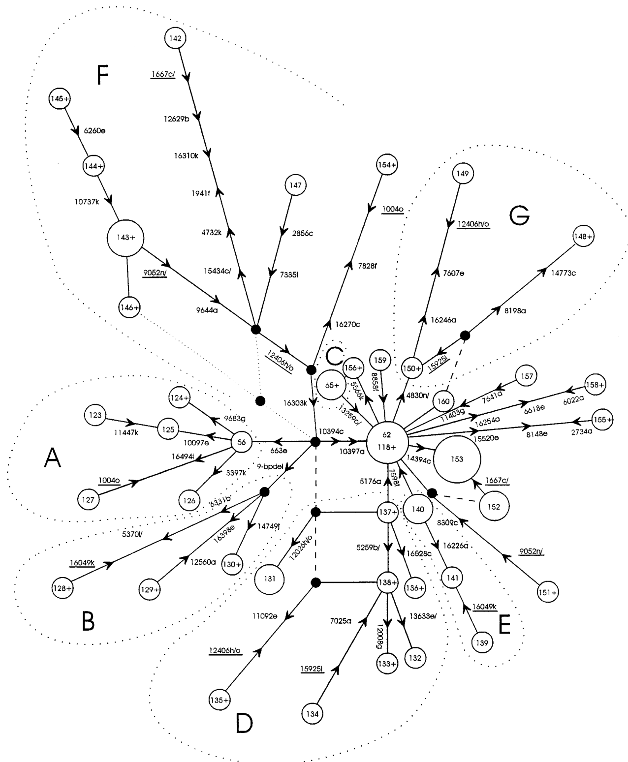
FIG. 6.—MJ network ( \epsilon = 0 ) for Tibetans, based on mtDNA restriction sites (Torrioni et al. 1994; sites 10394 Dde I and 10397 Alu I are weighted 1/2; site 16517 Hae III is disregarded, but its presence is indicated by “+” accompanying the sequence types; an error in the original table concerning the status of 10394 Dde I/10397 Alu I in mtDNA type 118 has been corrected). Designation of sequence types, restriction sites, and mtDNA groups A to G accords with Torrioni et al (1994). A slash indicates that a site is recognized by more than one restriction enzyme, and underlining denotes resolved recurrent mutations. Arrows point to presence of restriction sites; areas of circles are proportional to the numbers of sampled individuals. The dotted links do not appear in any MP trees; the unbroken links indicate a plausible MP tree (see text).
